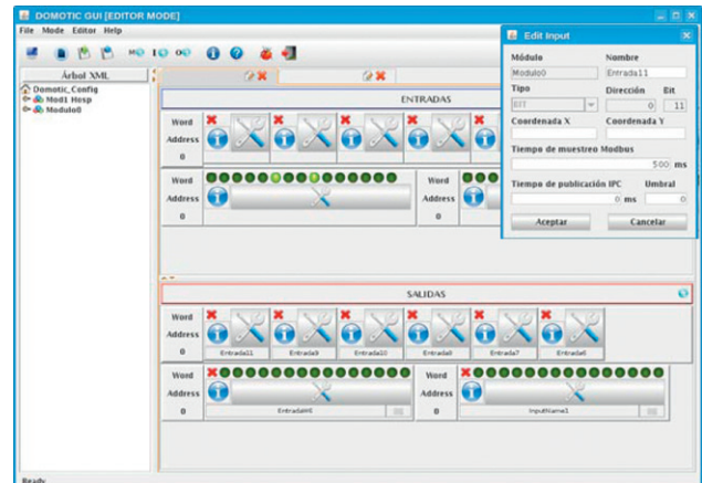
Figura 10: Ventana principal de Building Interface GUI.
