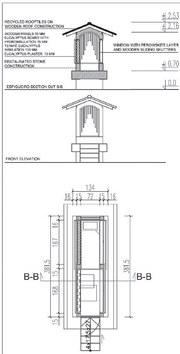
Figure 11 | Technical drawing with a proposition of reusing a granary as a single person sleeping unit on Camino de Santiago pilgrimage trail, author M.Orszt.
