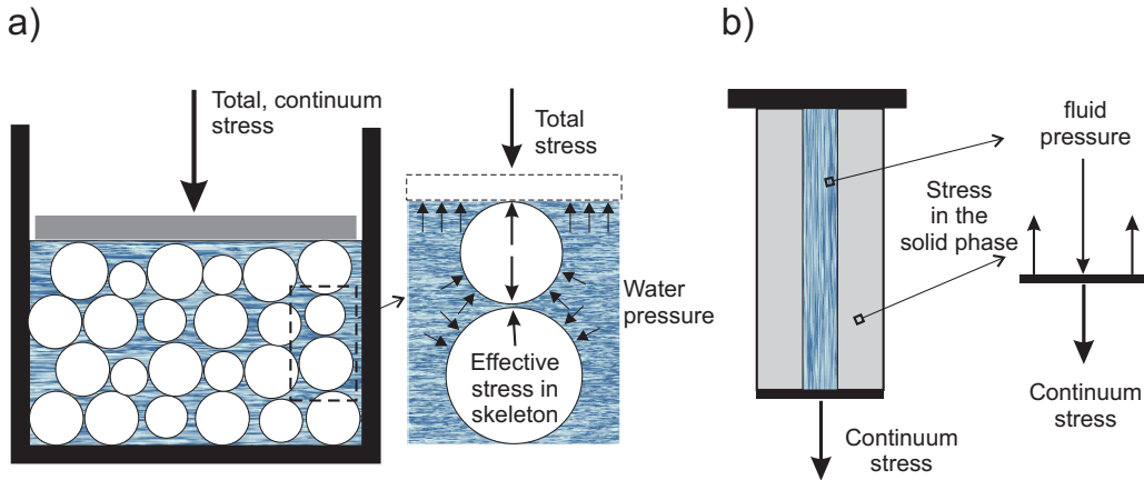
Figure 1: (a) The concept of effective stress in the soil skeleton. (b) Stress in the solid phase upon an increase of fluid pressure
