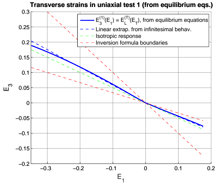
Figure 3: Transverse-to-axial strains E_3(E_1) \equiv E_L(E_T) obtained as a part of the strain energy determination procedure. Axis 3 corresponds to the fibre direction and axis 1 corresponds to the cross-fibre direction. The slope, at each strain value, is (minus) the equivalent instantaneous Poisson's ratio defined in terms of logarithmic strains, which is obtained by compatibility from the computed solution
