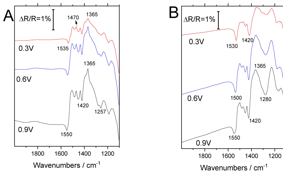
Figure 3. In situ FTIR spectra collected in PBS- \text{D}_2\text{O} for (A) PEDOT and (B) PHMeEDOT electrodeposited films. Sample potentials are indicated in the figure. The reference spectra were obtained at 0.1 V and 100 interferograms were collected at each potential.
