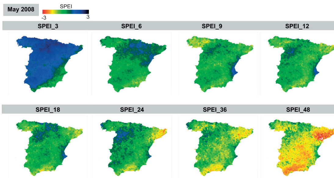
Figure 1. Series of timescales computed for a given month (May 2008) showing the spatial distribution of drought.
